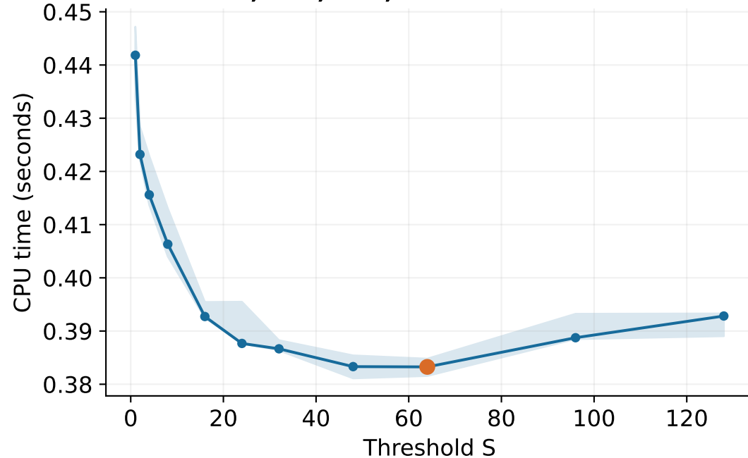
n = 10,000,000; coarse winner S=64
