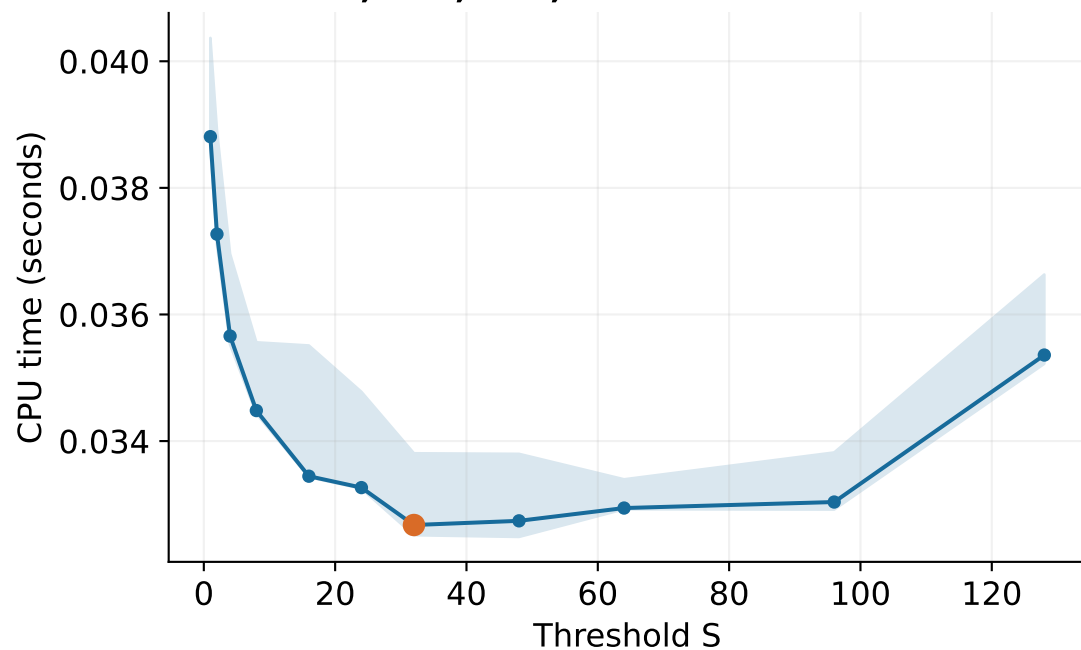
n = 1,000,000; coarse winner S=32
